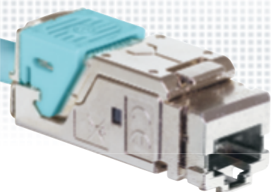
Cat. 8 toolless connector: up to 2500 connection/disconnection cycles
